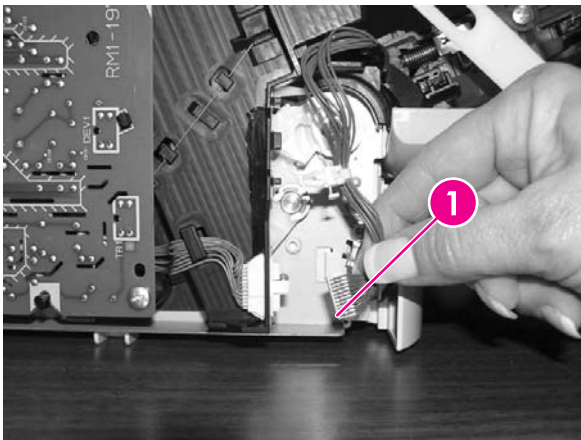
ETB connector
